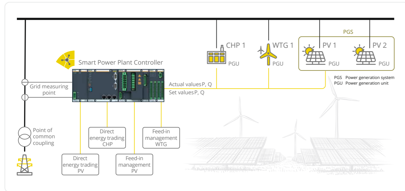
Example of a plant structure with smart power plant controller
